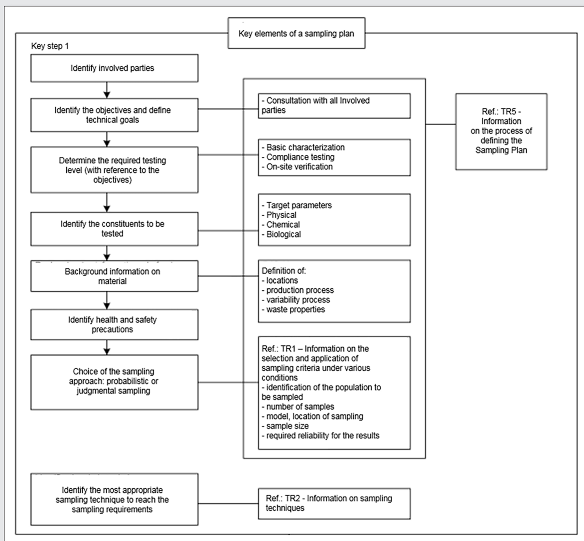
Figure 2. Key elements of a sampling plan following EN 14899.
